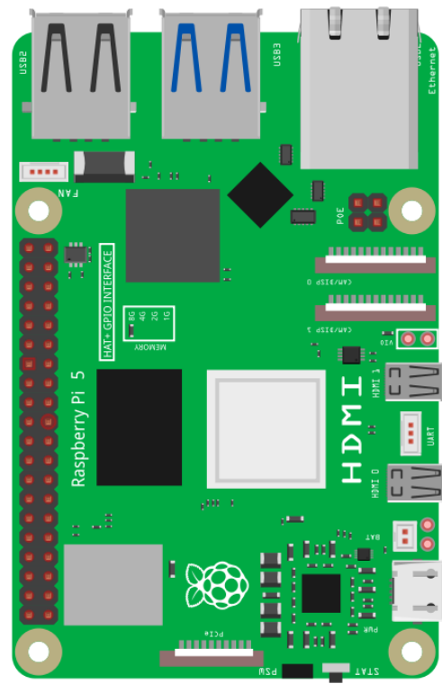
Model diagram of Raspberry Pi 5:
